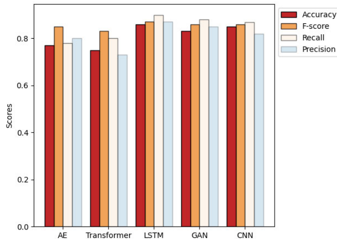
Figure 5. Detection Results of Models on KPI Data
