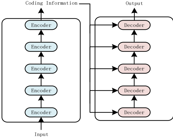
Figure 1. Transformer Brief diagram of the structure
