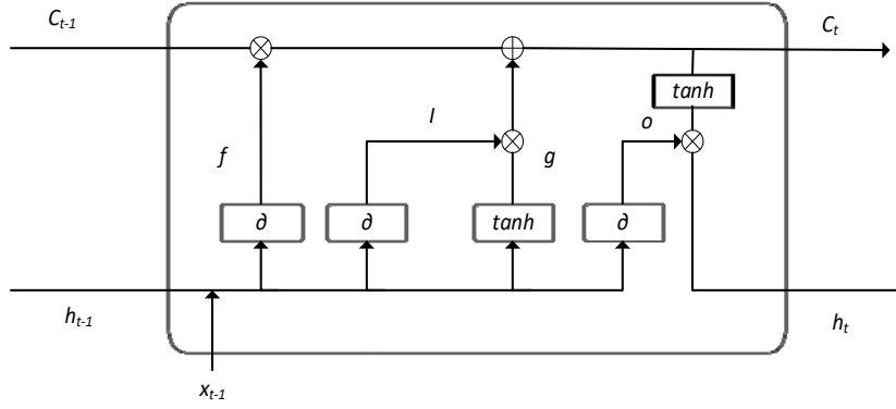
Figure 3. Structural diagram of the LSTM cells
